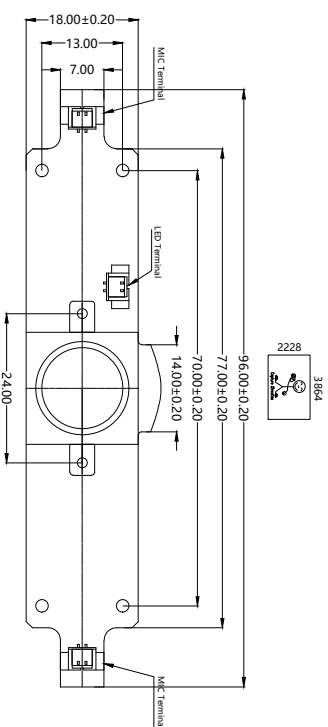
TOP VIEW
